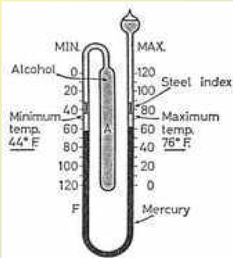
Six-Bellani termomeeter
